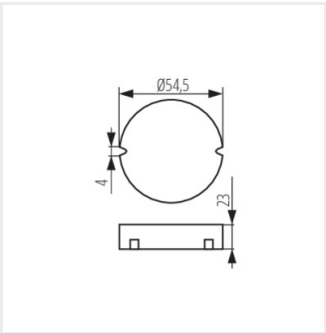
CIRCO N LED 12VDC
