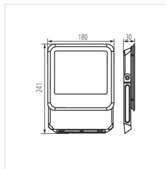
IQ-LED FL-50W-NW
