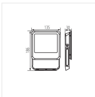
IQ-LED FL-30W-NW
