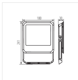
IQ-LED FL-50W-NW
