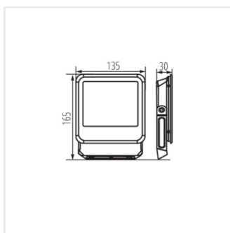
IQ-LED FL-20W-NW
