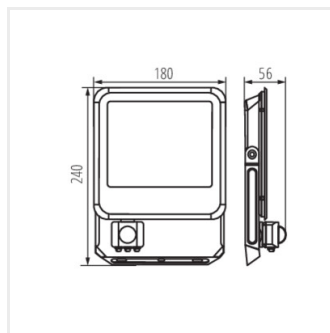
IQ-LED FL-50W-NW-SE
