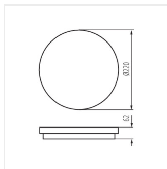
STIVI LED 10W; 15W
