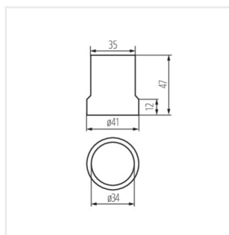
HLDR-E27
