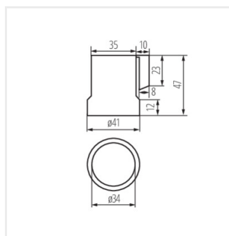
HLDR-E27-F
